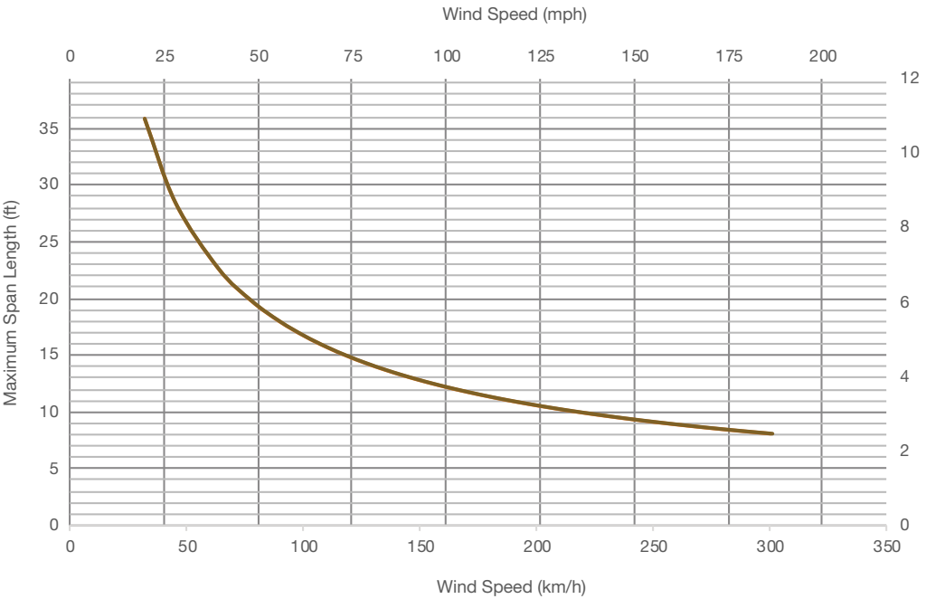
Span length for wind on narrow side
