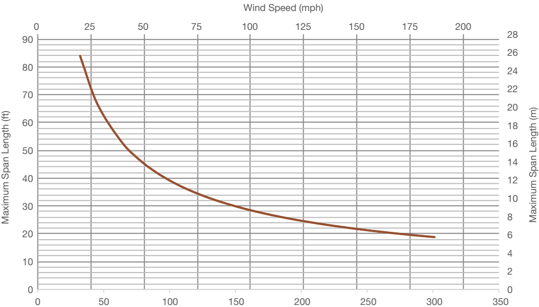
Span length for wind on narrow side
