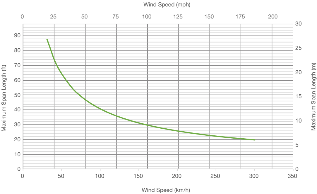
Span length for wind
