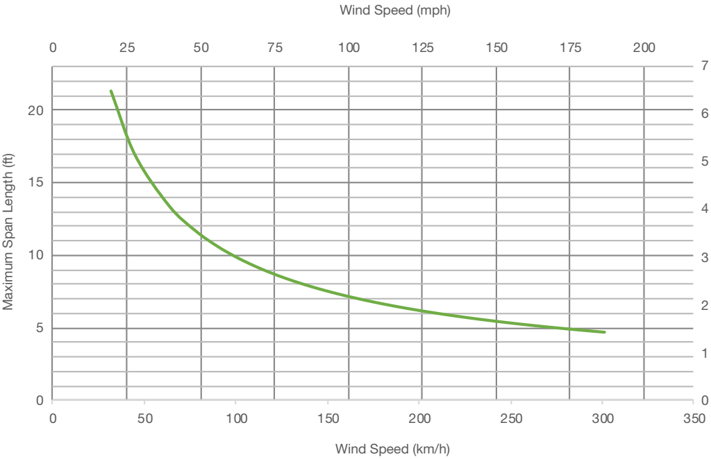
Span length for wind on wide side
