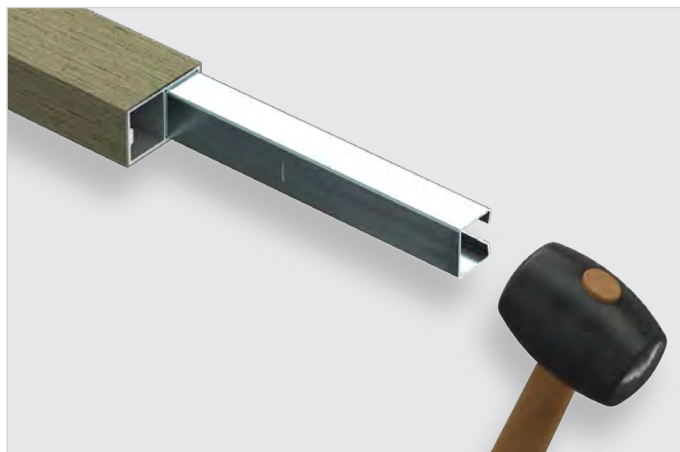
Install the connector using a mallet.
