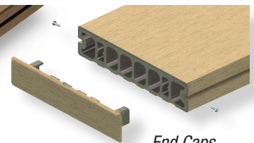
End Caps and Screws
