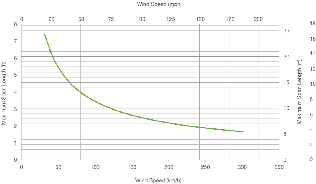
Span length for wind on wide side
