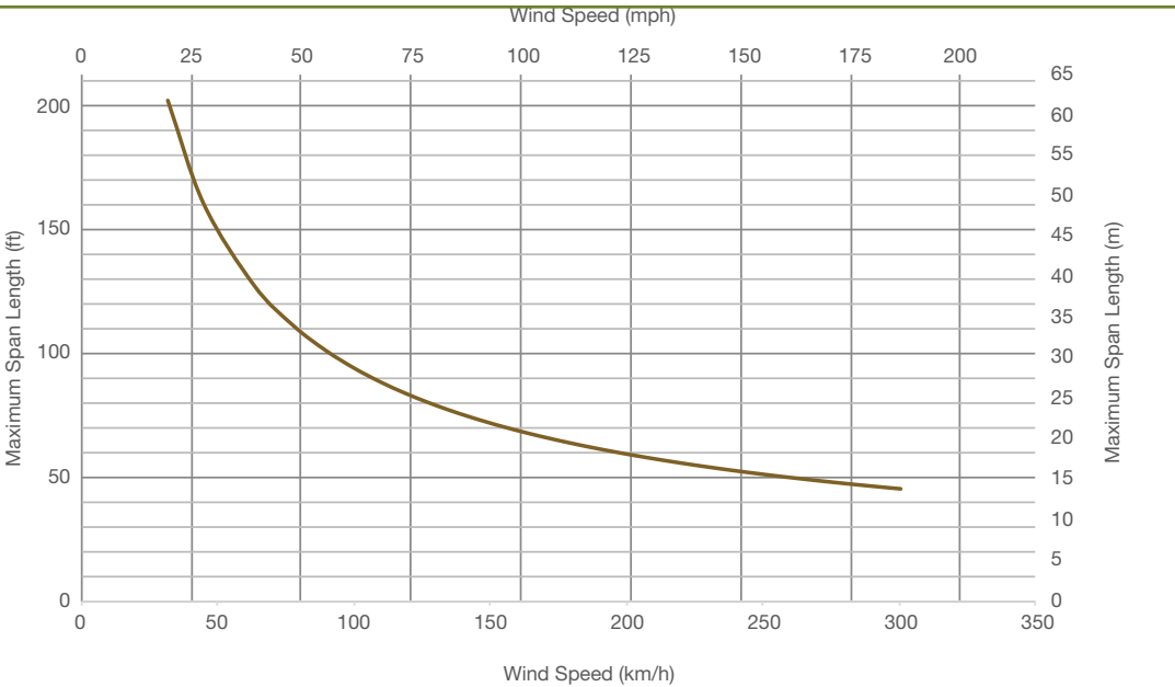
Span length for wind on narrow side
