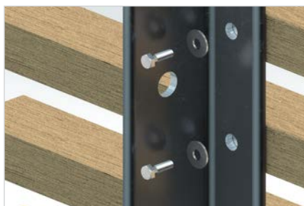
Installation of the supporting structure. The pre-drilled holes are wider (2 to 4 mm) than the bolt shaft to allow for expansion of the board. Washers are required as shown.
